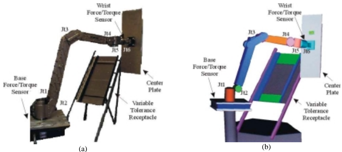
Figure 4 – Real (a) and Simulated (b) Experimental System
