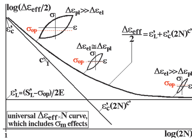
Figure 3: Universal \Delta\varepsilon_{eff} \times N curve, which describes fatigue lives under any mean load.
