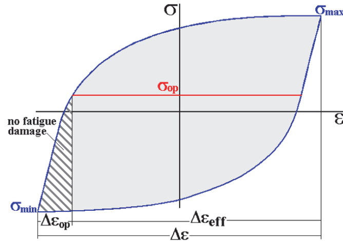
Figure 2: The effective strain range of the hysteresis loop, \Delta\varepsilon_{eff} = \Delta\varepsilon - \Delta\varepsilon_{op} , is the loop portion where the microcrack is completely open, thus can suffer fatigue damage.
