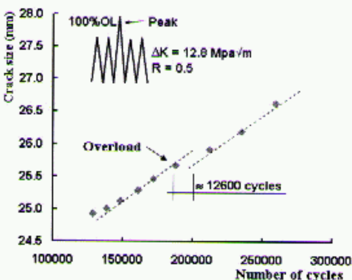
Figure 7. Fatigue crack growth retardation after a 100% overload, R = 0.5 .
