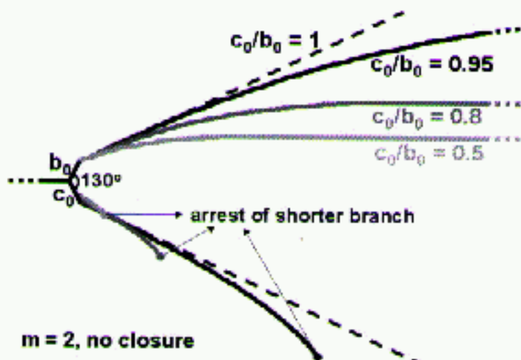
Figure 5. Bifurcated crack paths for several c_0/b_0 ratios.
