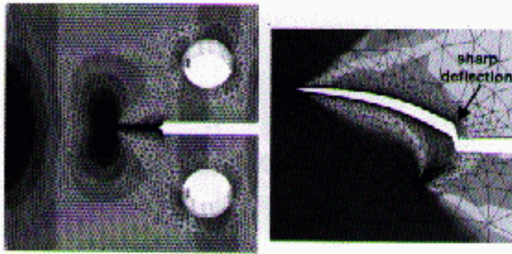
Figure 4. Propagation simulation of a bifurcated crack on a CT specimen (left), with a close-up of the two original 11\mu\text{m} and 10\mu\text{m} branches with angle 2\theta = 150^\circ (right).
