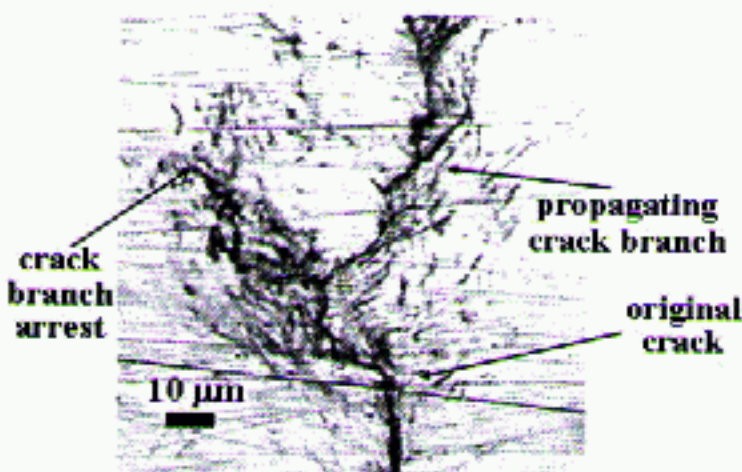
Figure 6. Crack branching on an SAE 4340 ESE(T) specimen.
